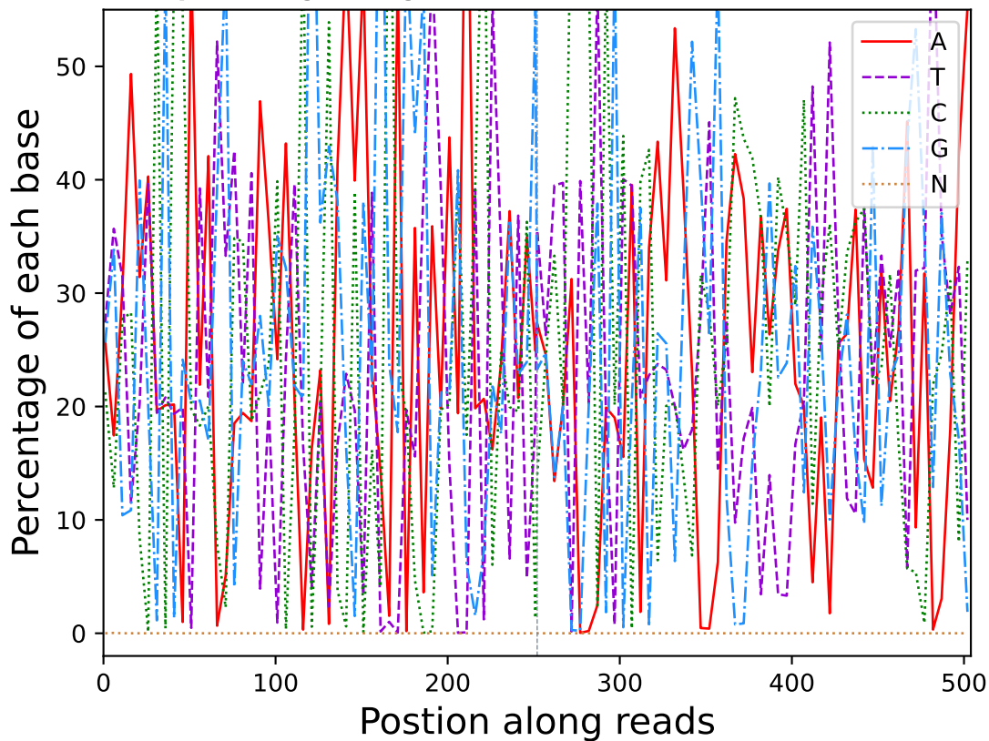
Base percentage along reads (R10917)
